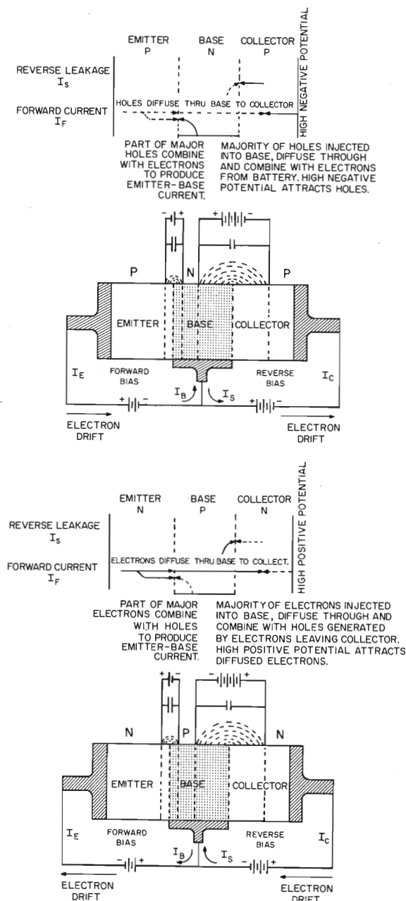
BIASED JUNCTION TRANSISTOR (COMMON BASE CONNECTION)
