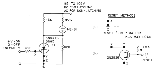
SCR REPLACEMENT
