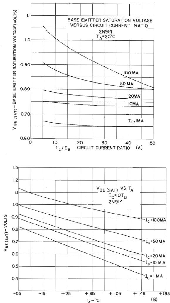
VARIATIONS IN V_{BE(SAT)} WITH OPERATING CONDITIONS Figure 6.9
