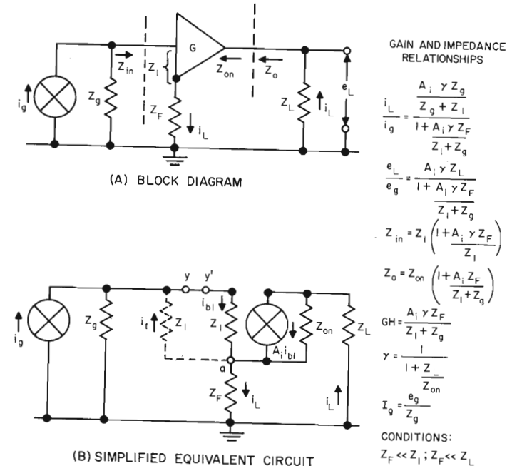
CURRENT FEEDBACK AMPLIFIER
