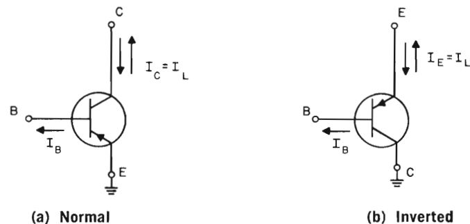
(a) Normal (b) Inverted THE NORMAL AND INVERTED CONNECTIONS
