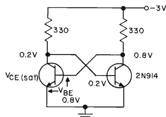
DIRECT COUPLED TRANSISTOR LOGIC (DCTL) FLIP-FLOP
