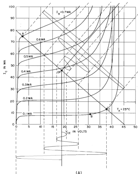
TYPICAL VI CHARACTERISTICS OF THE SILICON PLANAR 2N1613
