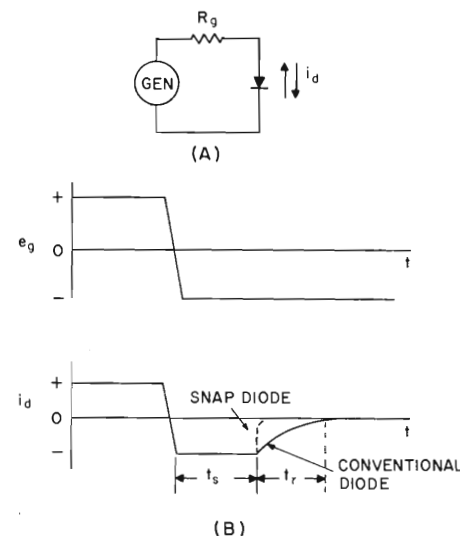
REVERSE RECOVERY OF A DIODE
