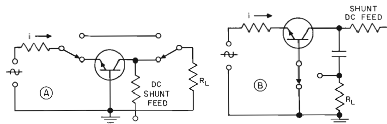
METHODS OF CALIBRATING UNITY CURRENT
