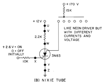
(B) NIXIE TUBE
