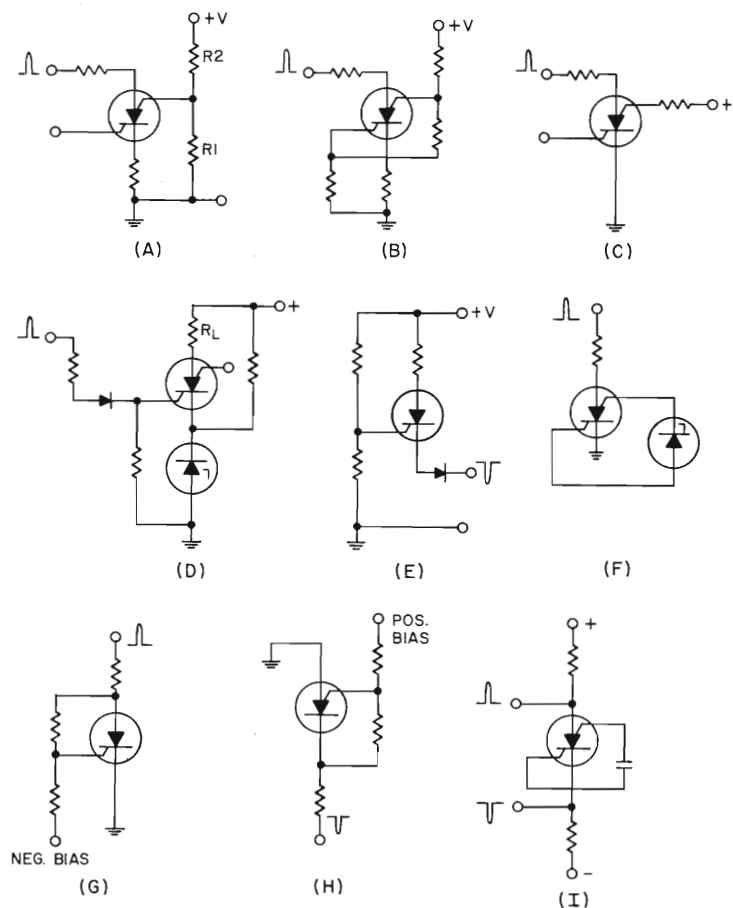
THRESHOLD CIRCUITS Figure 16.18
