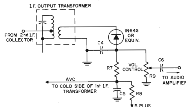
DETECTOR STAGE Figure 12.12
