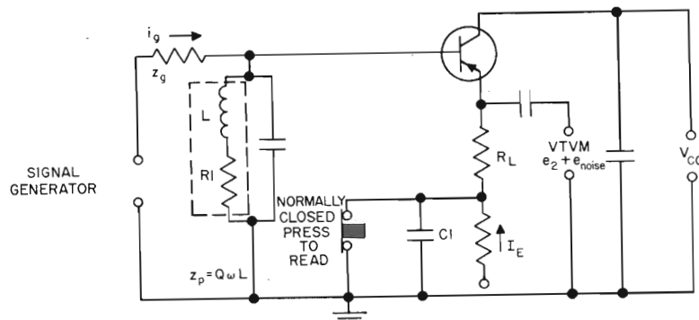
Figure 18.38 h_{re} MEASUREMENT
