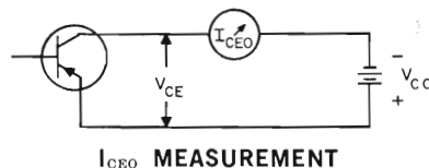
I_{CEO} MEASUREMENT Figure 18.5
