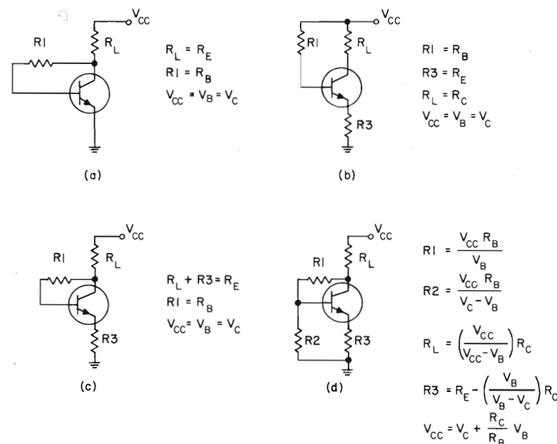
BIAS CIRCUIT VALUES IN TERMS OF GENERAL BIAS PARAMETERS
