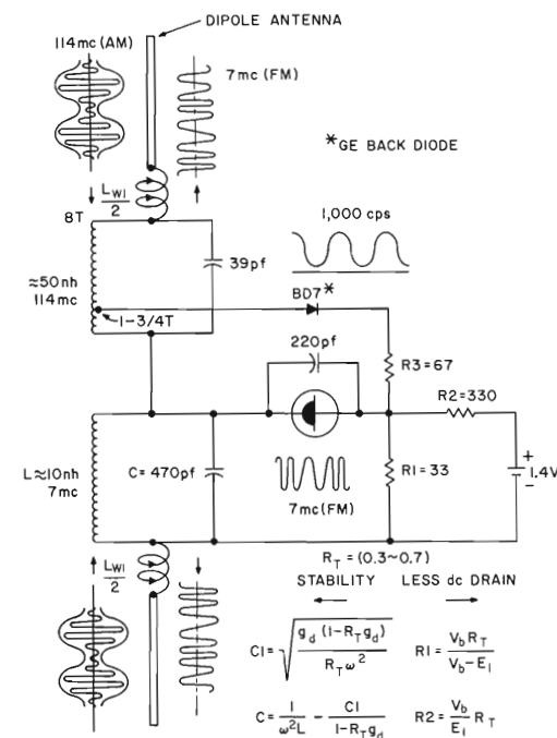
Figure 14.24 TUNNEL DIODE TRANSCIVER (19)
