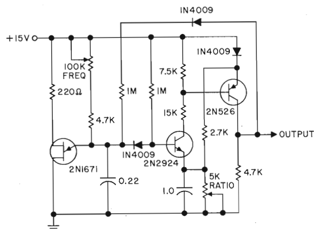
PULSE GENERATOR (VARIABLE FREQUENCY AND DUTY CYCLE)
