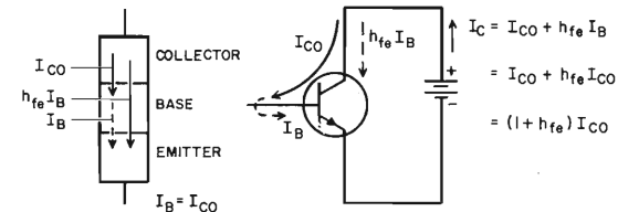
EFFECT OF TRANSISTOR GAIN ON LEAKAGE CURRENT
