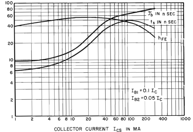
Figure 6.20 VARIATION OF \tau_b , t_s , AND h_{FE} WITH I_C
