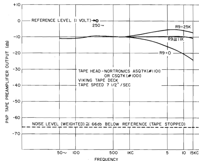
TAPE PREAMPLIFIER RESPONSE FROM NAB RECORDING Figure 11.19
