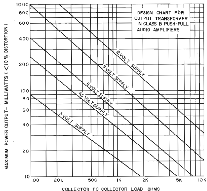
DESIGN CHART FOR OUTPUT TRANSFORMER IN CLASS B PUSH-PULL AUDIO AMPLIFIERS
