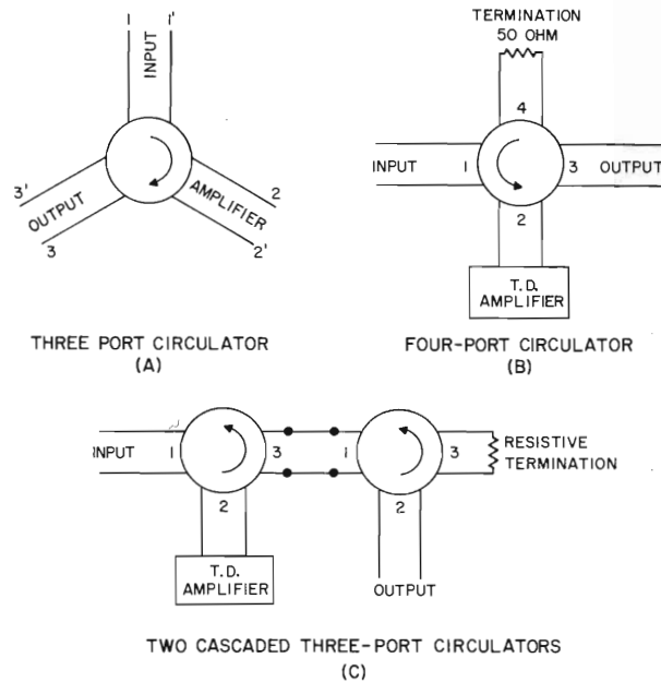
TUNNEL DIODE UHF CIRCULATORS Figure 14.29
