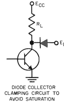
COLLECTOR VOLTAGE CLAMP Figure 6.22
