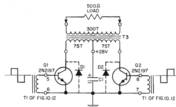
DC TO AC (SQUARE WAVE) INVERTER Figure 10.11
