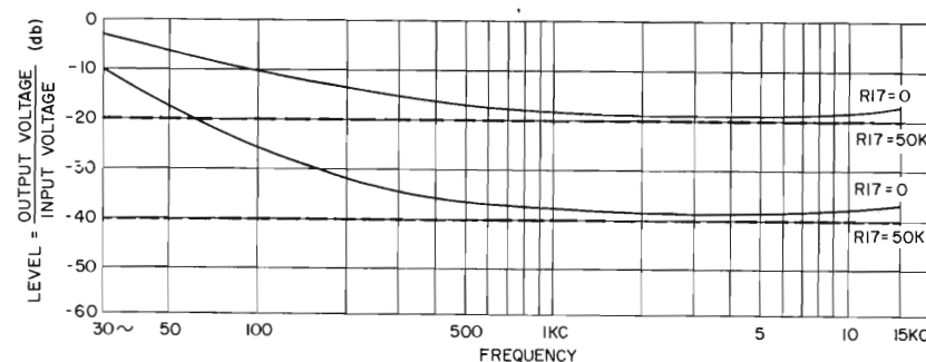
FREQUENCY RESPONSE OF BASS BOOST CIRCUIT
