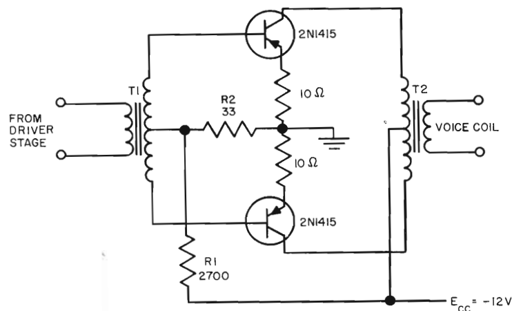
CLASS B PUSH-PULL OUTPUT STAGE
