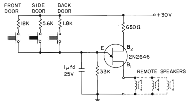
UNIJUNCTION HOME SIGNAL SYSTEM
