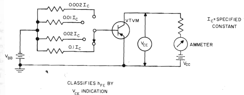
h_{FE} CLASSIFIER
