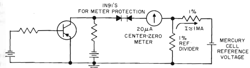
V_{CE(SAT)} MEASUREMENT
