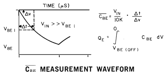
\overline{C_{BE}} MEASUREMENT WAVEFORM Figure 18.69
