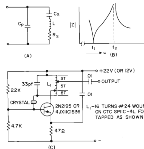
CRYSTAL OSCILLATOR
