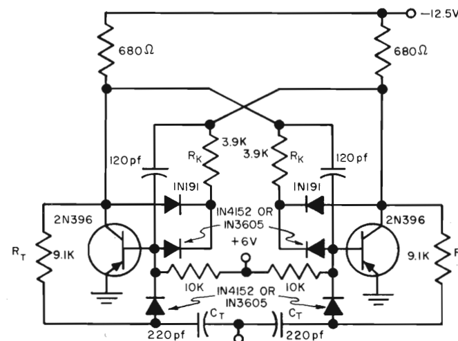
BASE TRIGGERING WITH HYBRID GATE Figure 7.17
