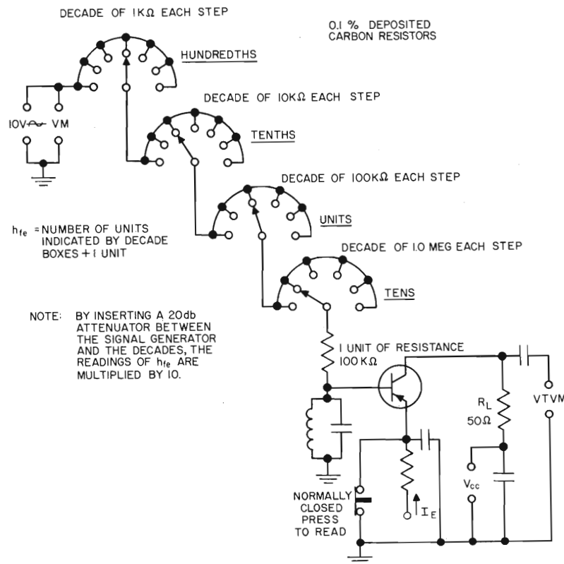
ALTERNATE h_{fe} MEASUREMENT
