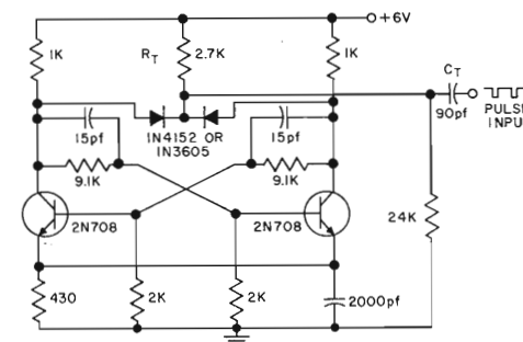
COLLECTOR TRIGGERING Figure 7.13
