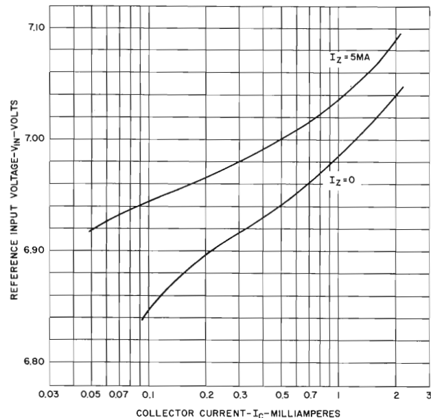
TRANSFER CHARACTERISTICS OF REFERENCE AMPLIFIER
