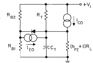
EQUIVALENT CIRCUIT FOR CALCULATION OF TEMPERATURE AND LOADING EFFECTS
