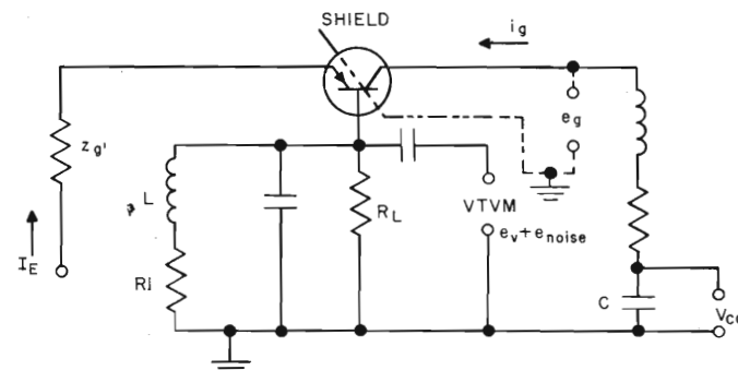
Figure 18.32 h_{ob} MEASUREMENT
