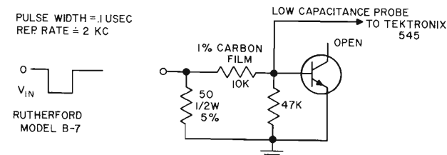
Figure 18.68 \overline{C_{BE}} TEST CIRCUIT
