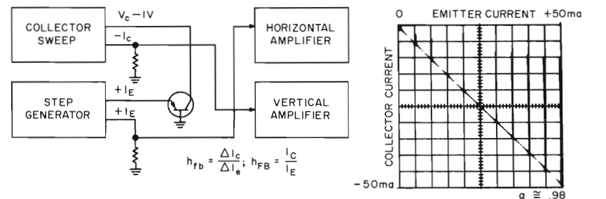
(E) ALPHA CURVE, \alpha , h_{21b} , h_{fb} , h_{FB}
