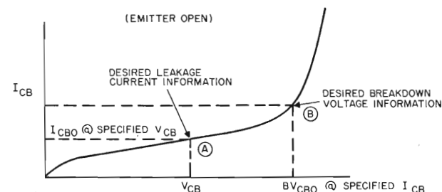
REPRESENTATIVE COLLECTOR-BASE JUNCTION REVERSE CHARACTERISTICS
