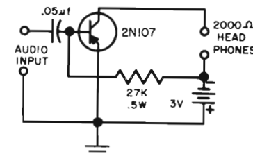
SIMPLE AUDIO AMPLIFIER
