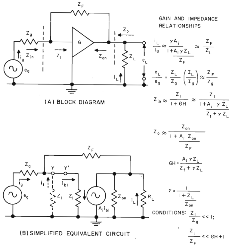
VOLTAGE FEEDBACK AMPLIFIER
