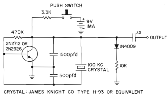
100 KC CRYSTAL STANDARD Figure 15.15
