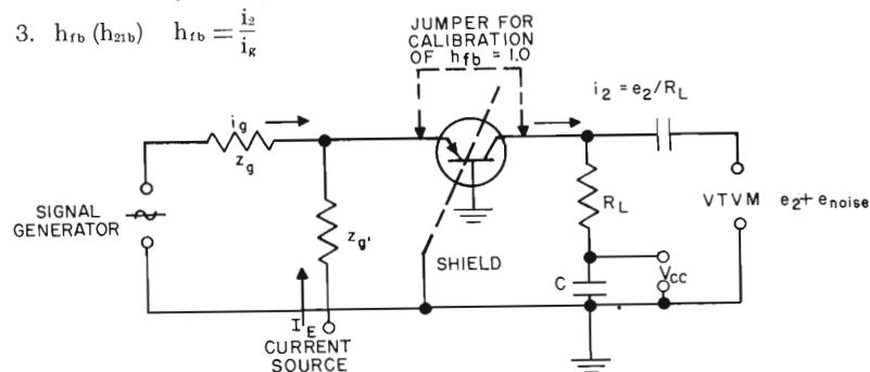
Figure 18.31 h_{fb} MEASUREMENT
