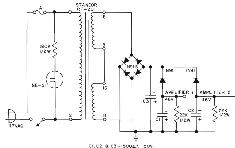
POWER SUPPLY FOR STEREO SYSTEM Figure 11.28
