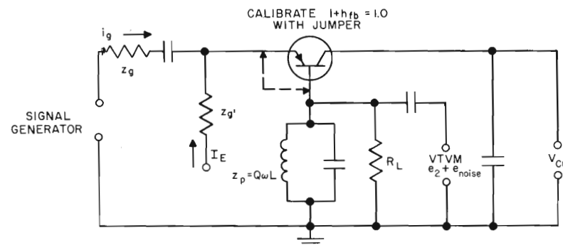
1 + h_{fb} MEASUREMENT
