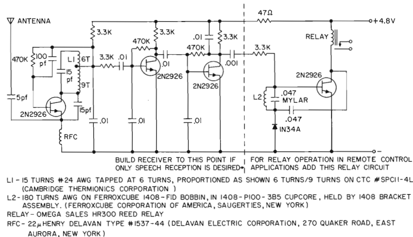
SUPERREGENERATIVE 27 MC RECEIVER
