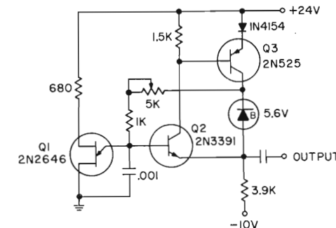
50 KC SAWTOOTH GENERATOR
