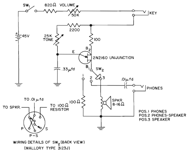
UNIUNCTION TRANSISTOR CODE PRACTICE OSCILLATOR
