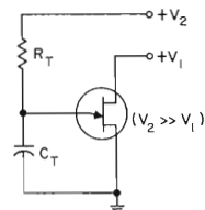
(A) USE OF HIGH VOLTAGE SUPPLY FOR CHARGING OF TIMING CAPACITOR
