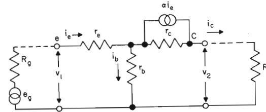
T-EQUIVALENT CIRCUIT (COMMON-BASE) WITH CURRENT GENERATOR Figure 2.3
