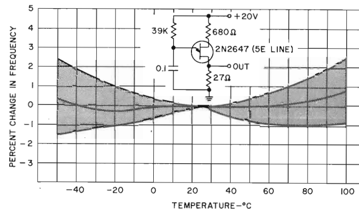
2N2647 TEMPERATURE CHARACTERISTIC
