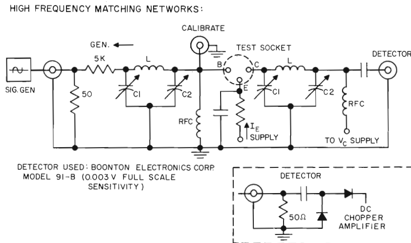
HIGH FREQUENCY POWER GAIN Figure 18.55
