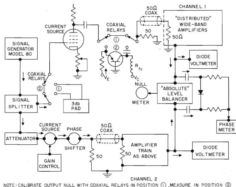
h_{rb} , f_{rb} AND PHASE OF \alpha MEASUREMENT UP TO 100 MCS
