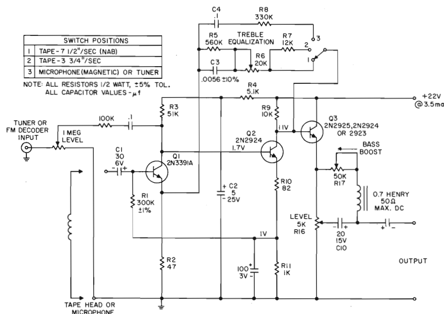
TAPE-MICROPHONE PREAMPLIFIER
