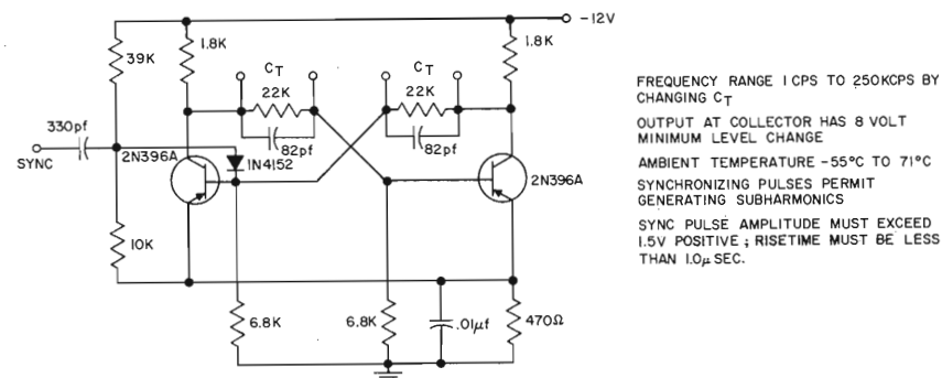
ASTABLE MULTIVIBRATOR
