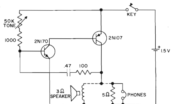
CODE PRACTICE OSCILLATOR
