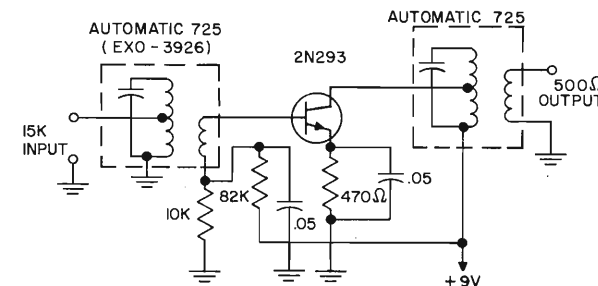
Figure 12.7 IF AMPLIFIER
