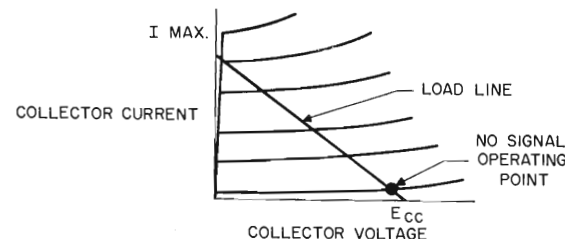
TYPICAL COLLECTOR CHARACTERISTICS AND LOAD LINE
