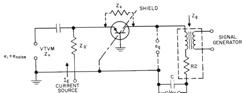
Figure 18.30 h_{fb} MEASUREMENT
