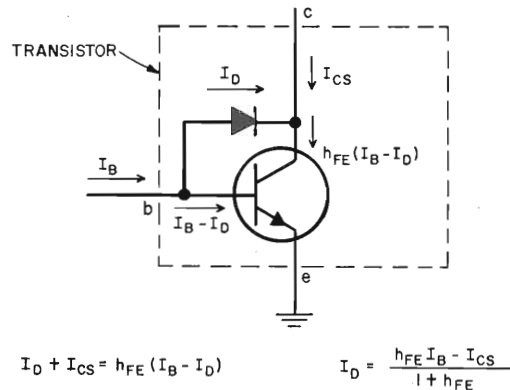
Figure 6.21 SIMPLE EQUIVALENT CIRCUIT FOR ESTIMATING STORAGE TIME WHEN APPRECIABLE CHARGE IS LOCATED IN COLLECTOR
