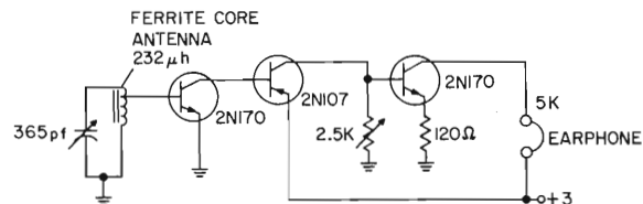
Figure 15.19 THREE TRANSISTOR RECEIVER (AM Broadcast Band)
