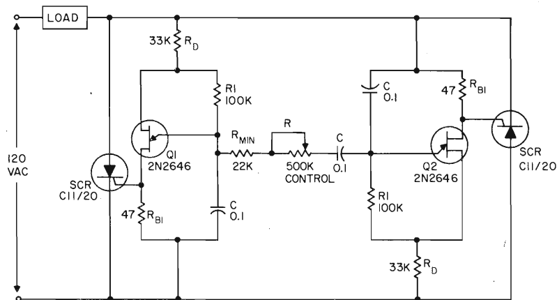
SIMPLIFIED FULL-WAVE UJT TRIGGER CIRCUIT
