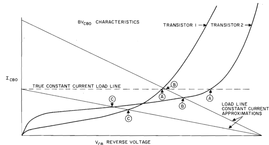
BV CBO MEASUREMENT TECHNIQUES
