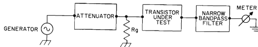
SET UP TO MEASURE (e_n^2)^{1/2} Figure 18.60
