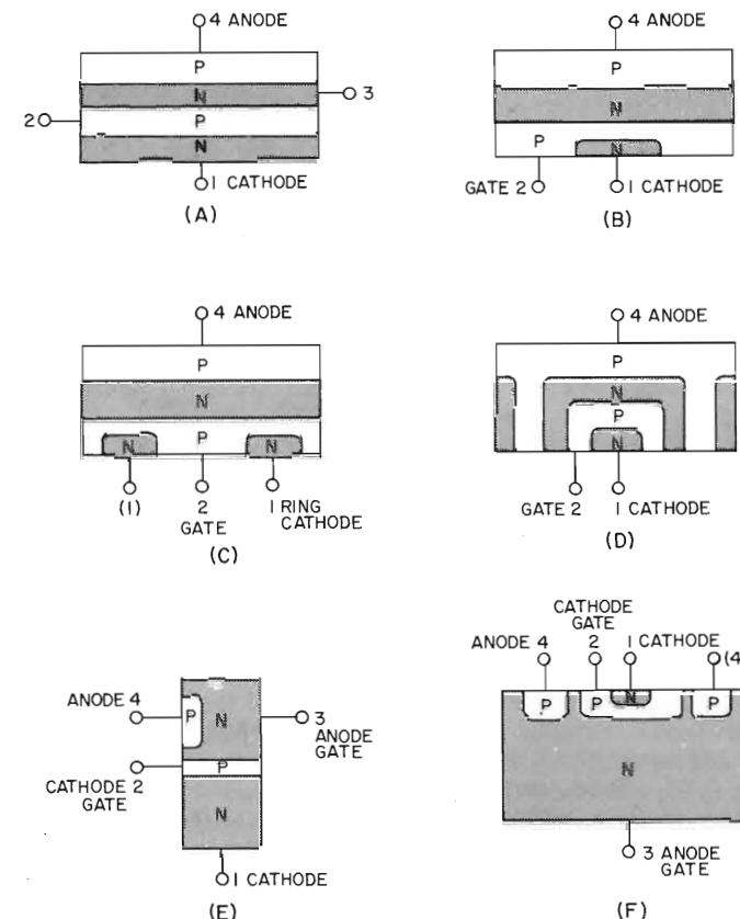
SECTIONAL VIEWS OF PNPN GEOMETRIES
