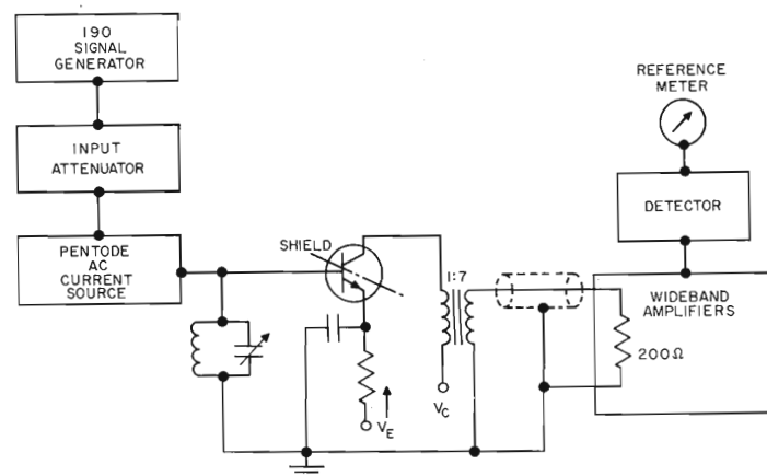
h_{fe} AND f_{ae} MEASUREMENT UP TO 10 MCS
