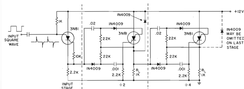
BINARY COUNTER
