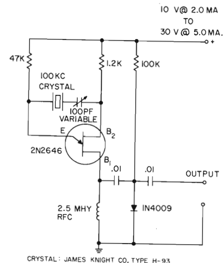
UNIUNCTION 100 KC CRYSTAL STANDARD Figure 15.16
