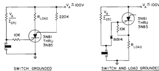
SWITCH OPENED TO TRIGGER SCS
